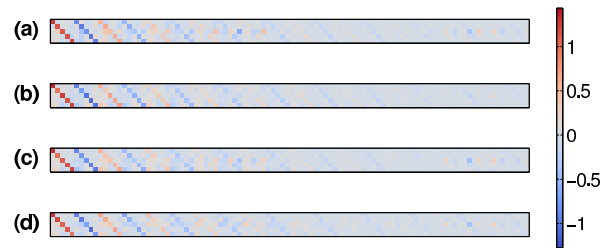
Fig. 3 Coefficient matrices of the first individualized model for each activity class: (a) forward, (b) rightward, (c) backward, and (d) leftward.
