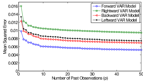
Fig. 2 Mean squared error as a function of lag.
