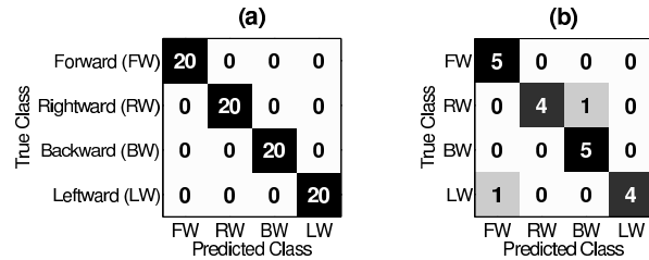
Fig. 6 Confusion matrices from testing the second individualized model on: (a) the training set and (b) the validation set.
