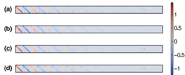
Fig. 7 Coefficient matrices of the combined model for each activity class: (a) forward, (b) rightward, (c) backward, and (d) leftward.
