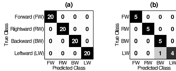
Fig. 4 Confusion matrices from testing the first individualized model on: (a) the training set and (b) the validation set.
