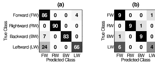
Fig. 8 Confusion matrices from testing the combined model on: (a) the training set and (b) validation set.
